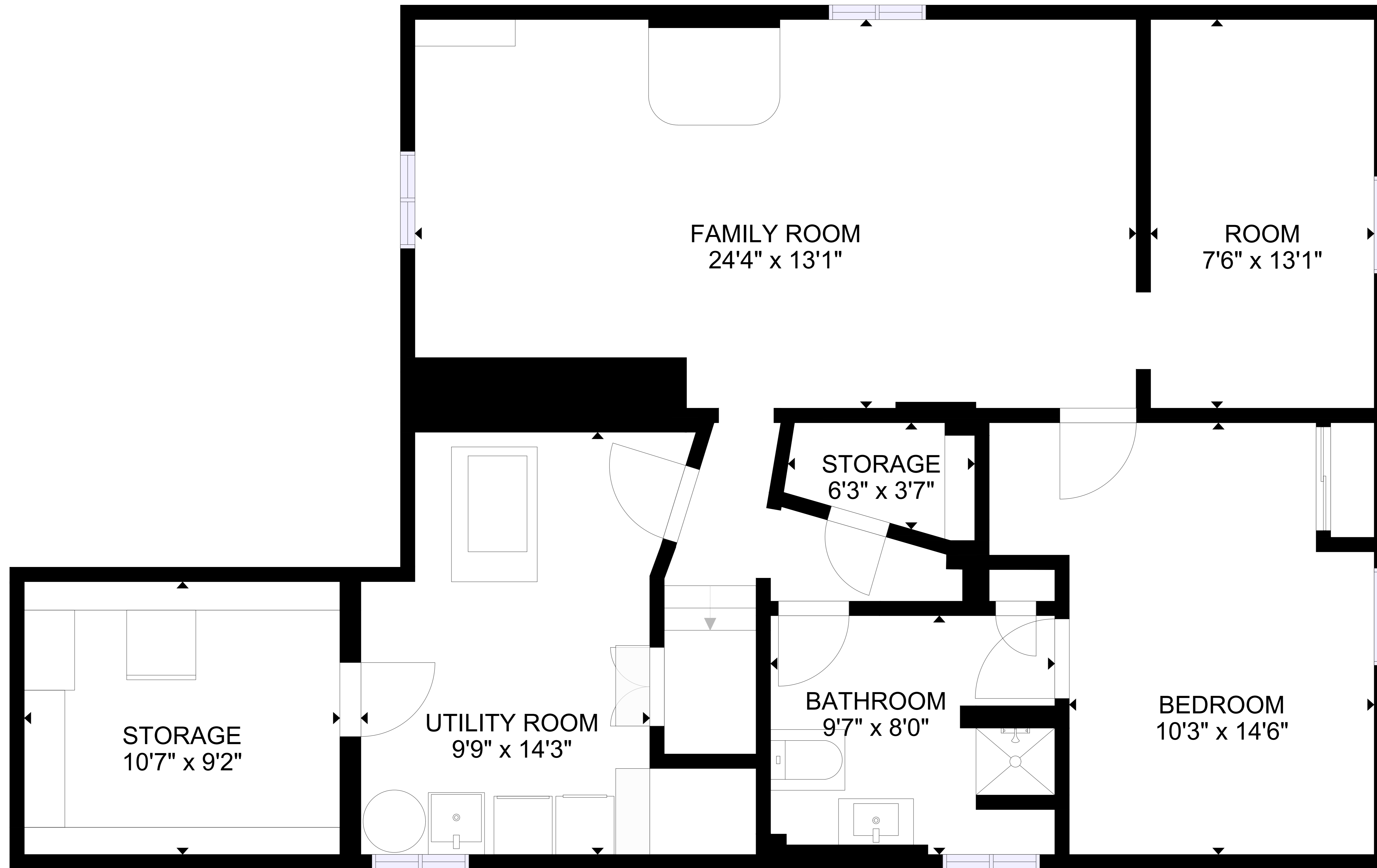
FLOOR 1
